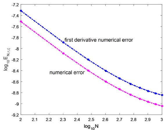
Figure 7. \log_{10} E1_{N,\tau,\xi} : \xi = 0.6, \tau = 0.0001
