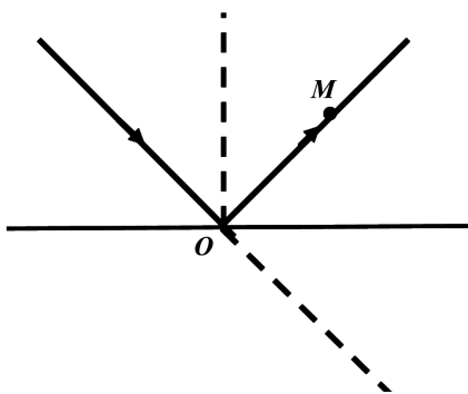
Figure 3. Specular reflection of light 图 3. 光的镜面反射图
