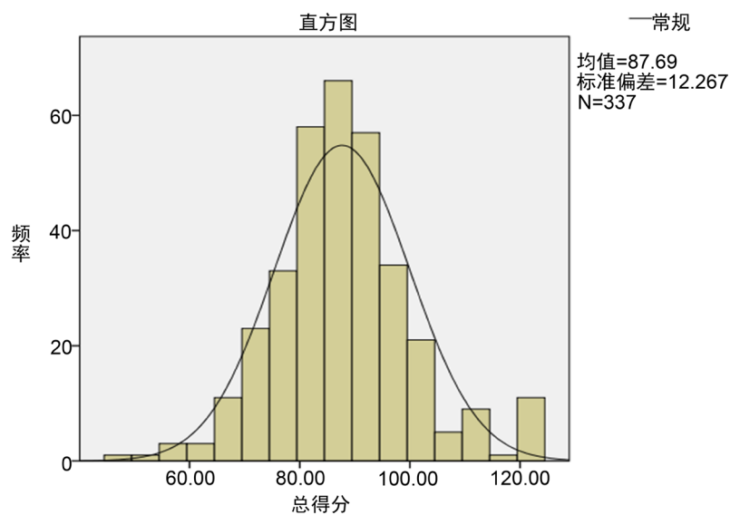
Figure 1. Histogram of total score frequency distribution
