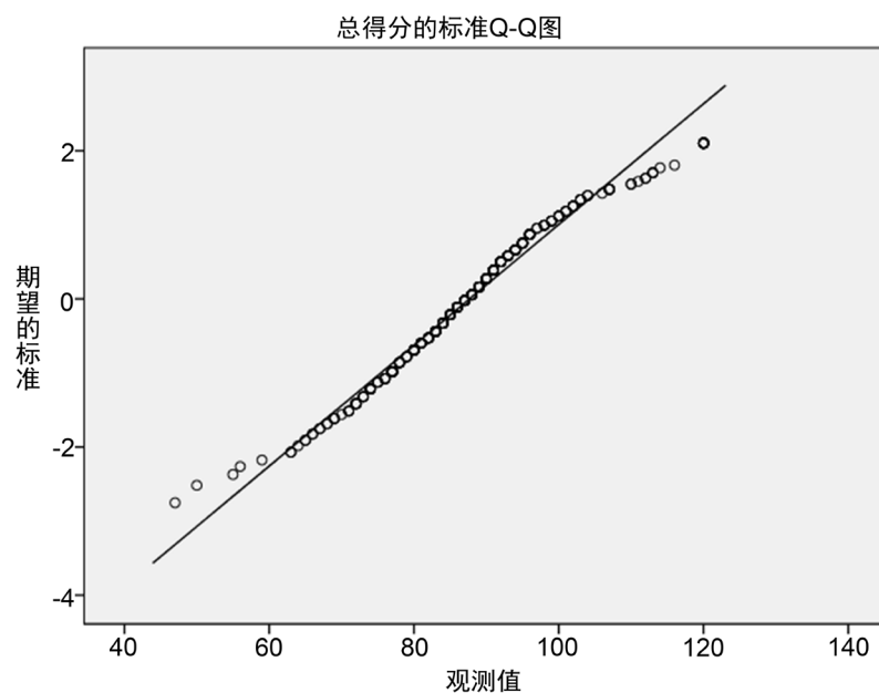
Figure 2. Standard Q-Q plot of total score
