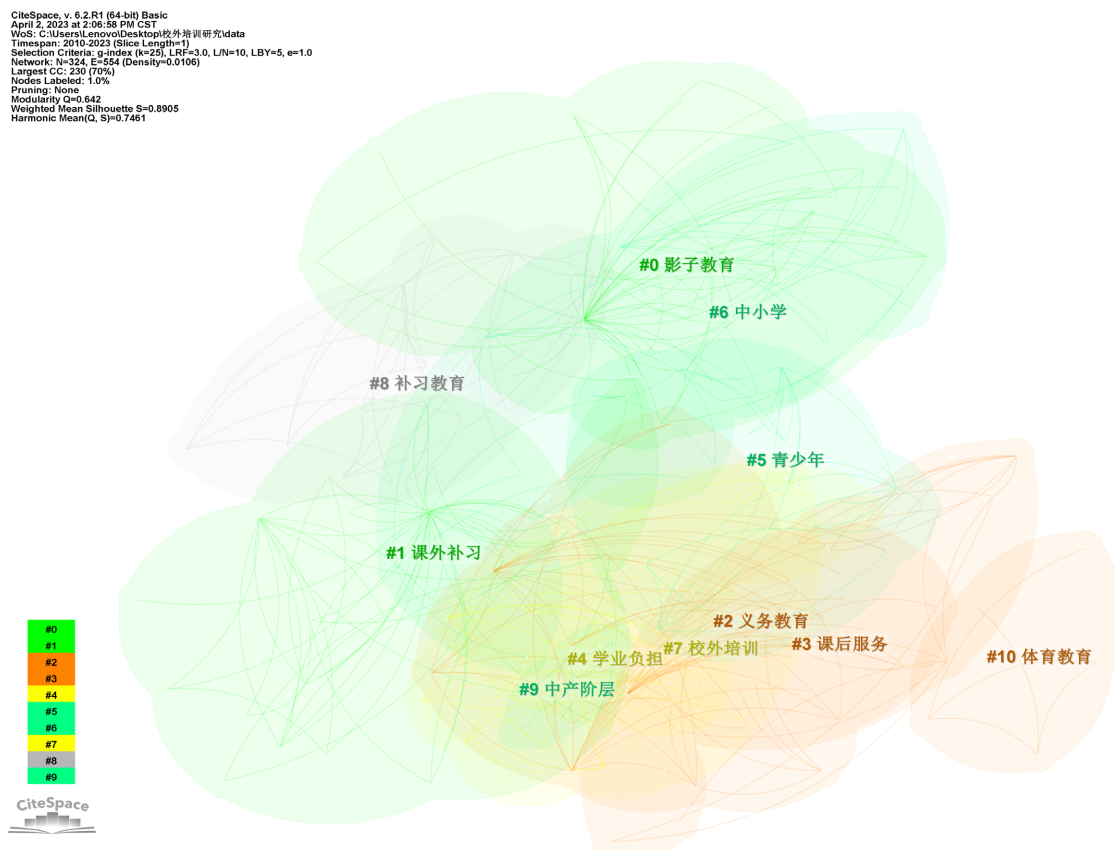
Figure 5. Keyword cluster graph
