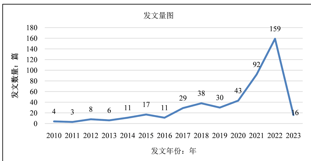
Figure 1. Statistics of annual publication volume
