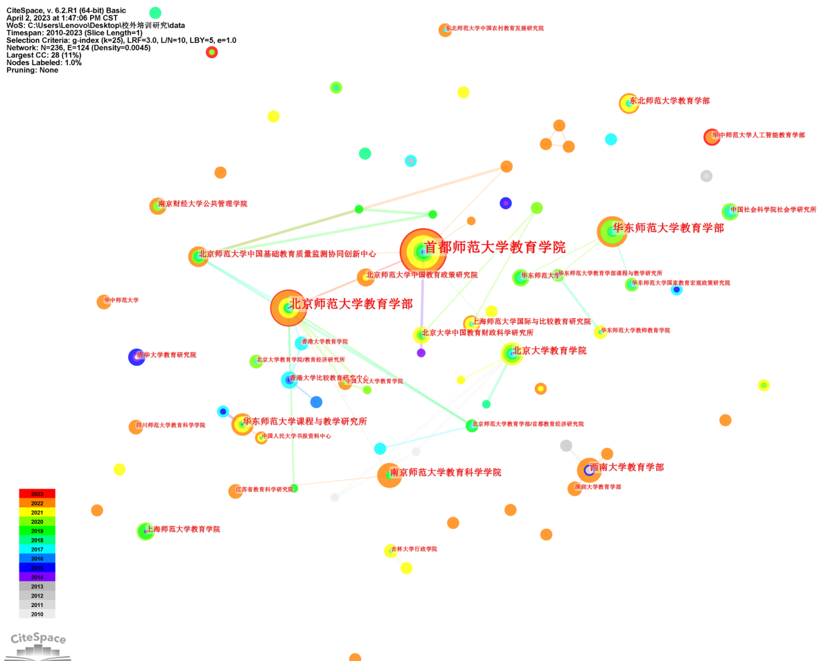
Figure 3. Research institution collaboration graph
