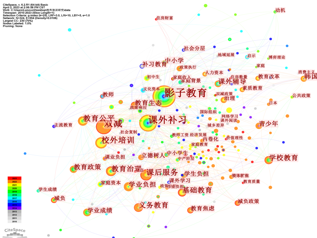
Figure 4. Keyword co-occurrence graph 图 4. 关键词共现图谱
