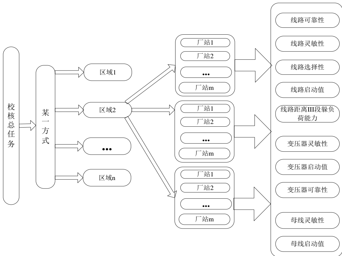
Figure 6. Sub-task division of parallel computing
