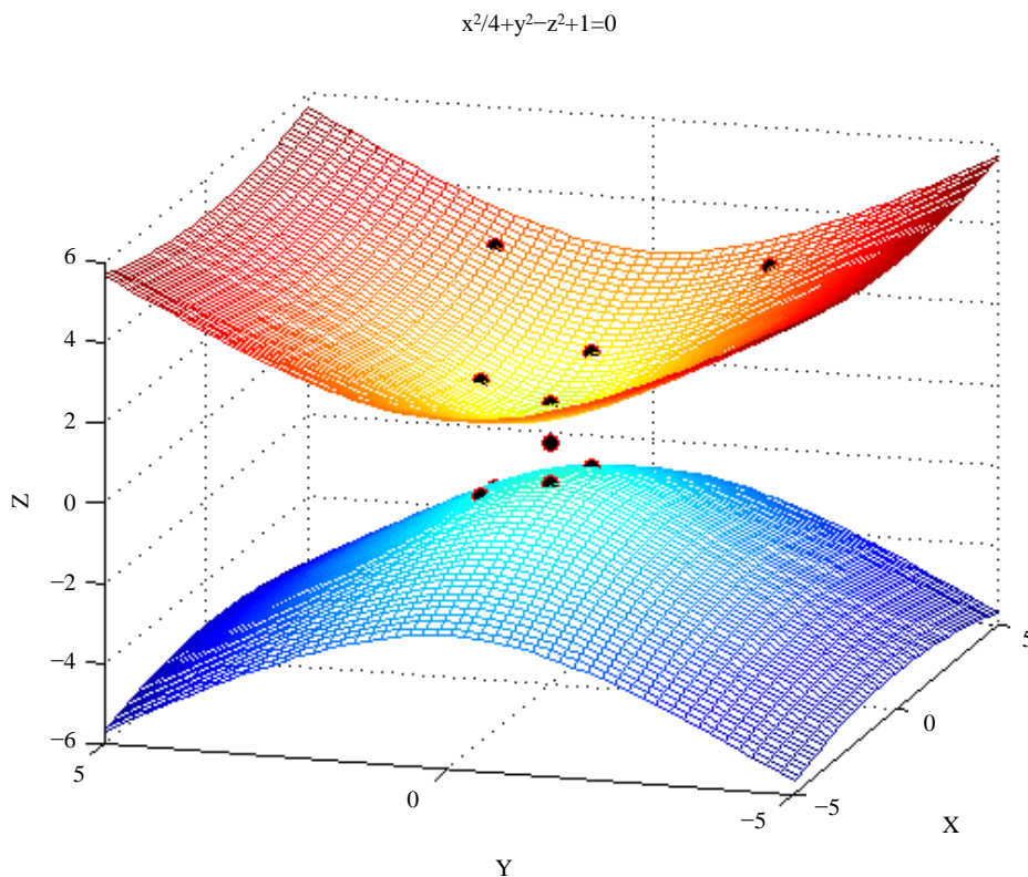
Figure 1. Point of the hyperboloid of two sheets 图 1. 双叶双曲面取点效果图
