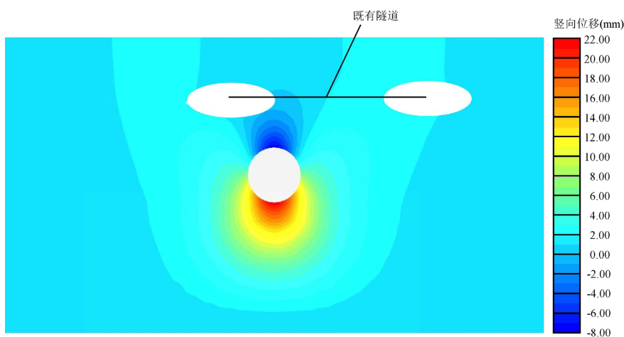
Figure 6. Contours of vertical displacement at profile of Ring 222 图 6. 222 环处竖向位移云图
