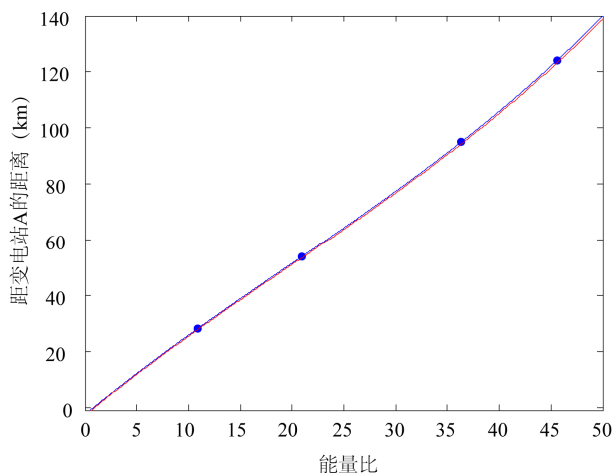
Figure 6. The energy ratio and the relationship curve 图 6. 能量比与距首端距离的关系曲线图
