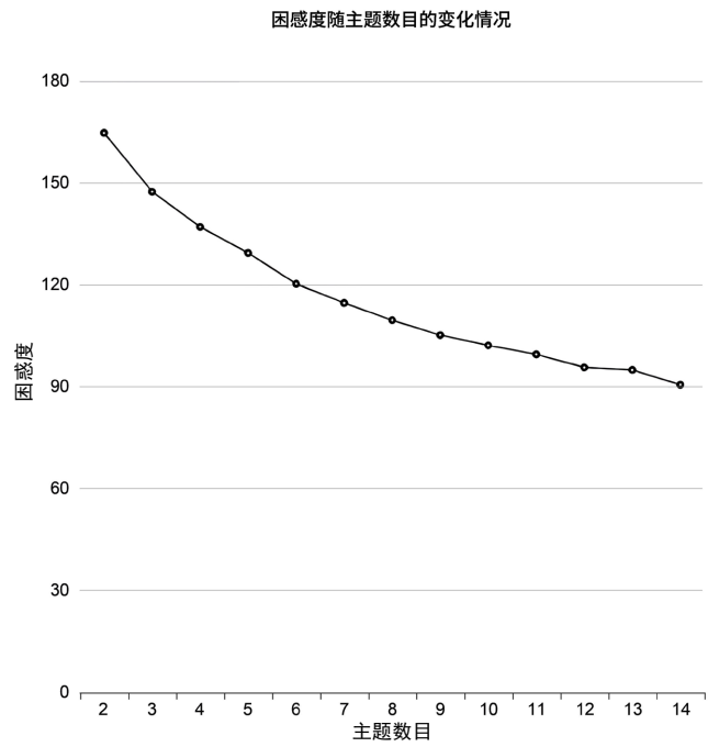
Figure 5. Variation of perplexity with the increase of topic numbers 图 5. 主题数目增加时的困惑度变化
