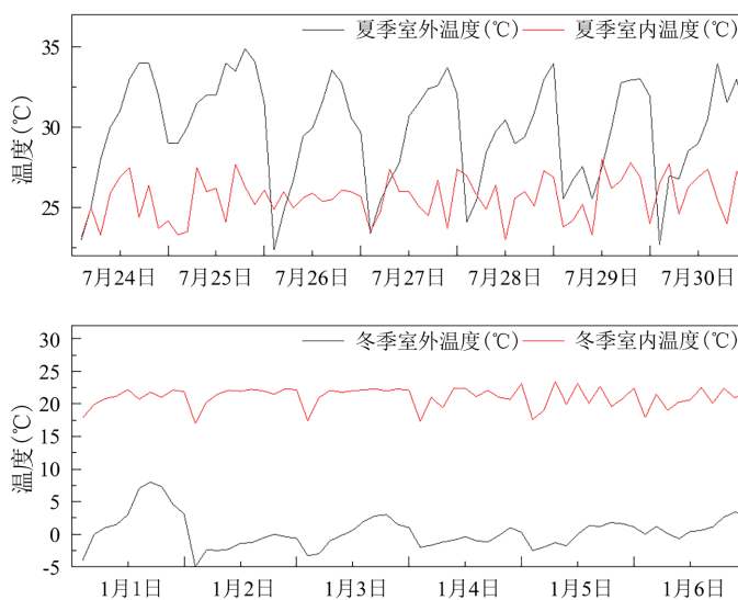
Figure 5. Temperature test results
