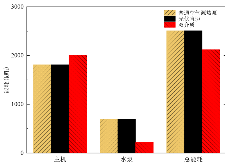
Figure 8. System energy consumption of three types of air source heat pumps
