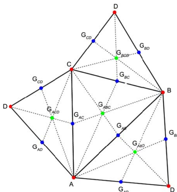
Figure 1. Symbolic expansion of point, line and surface 3-state barycentric coordinates 图 1. 点、线、面 3 态重心坐标符号展开图
