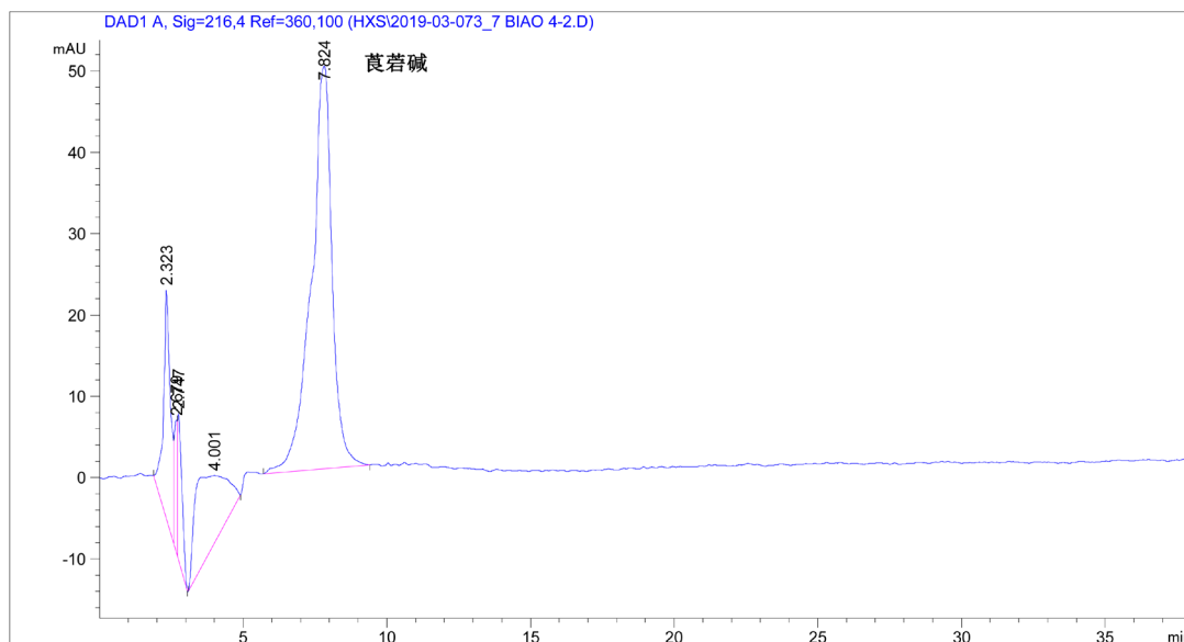
Figure 3. Standard chromatogram of hyoscyamine 图 3. 莨菪碱标准色谱图
