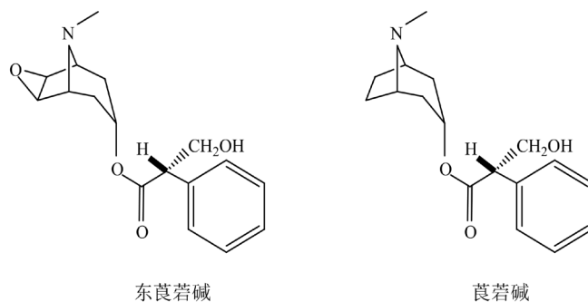
Figure 1. The chemical structures of scopolamine and hyoscyamine
