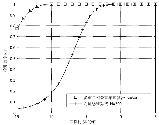
Figure 3. Simulation result when sampling point is 300 图 3. 采样点为 300 时的仿真结果
