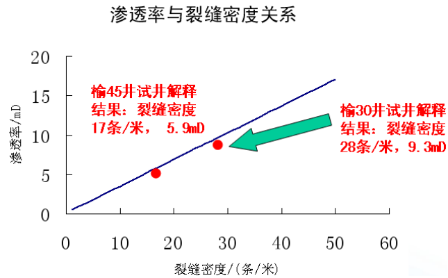
Figure 4. The relationship between permeability and the natural fracture density, the effective stress is 30 MPa 图 4. 渗透率与天然裂缝密度的关系，有效应力取 30 MPa
