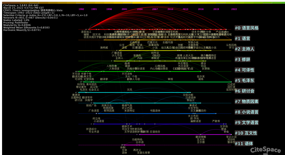
Figure 3. Keyword collinear time-line mapping 图 3. 关键词共线时间线图谱
