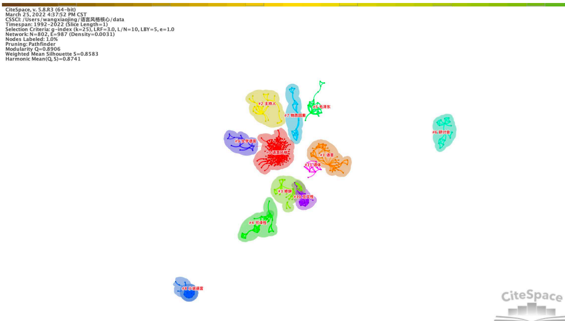
Figure 2. Keyword co-occurrence mapping 图 2. 关键词共现图谱
