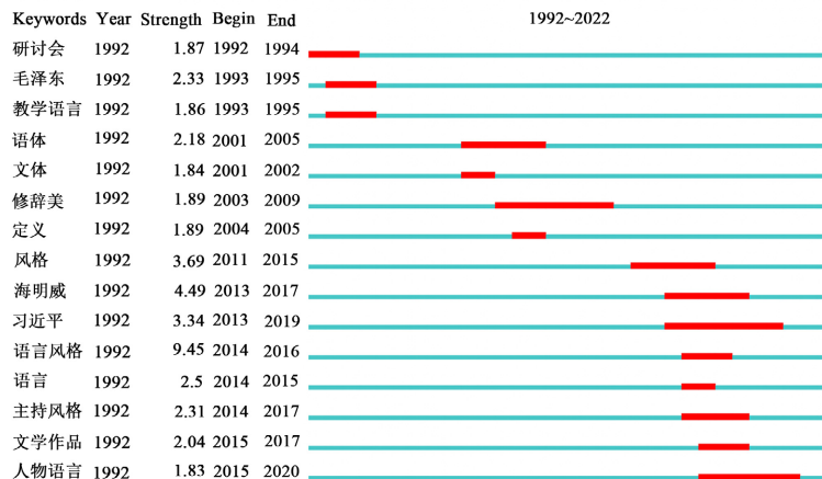
Figure 4. Burstiness mapping of language style studies in China (1992~2022) 图 4. 国内语言风格研究突现图(1992~2022)
