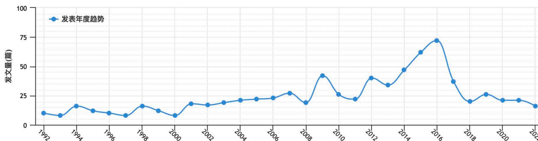
Figure 1. Number of language style research papers published in China in 1992~2022
