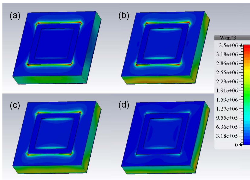
Figure 12. Power loss density distributions of microwave absorbing coatings at different frequencies (a) 3 GHz; (b) 8.7 GHz; (c) 10.6 GHz; (d) 15.4 GHz
