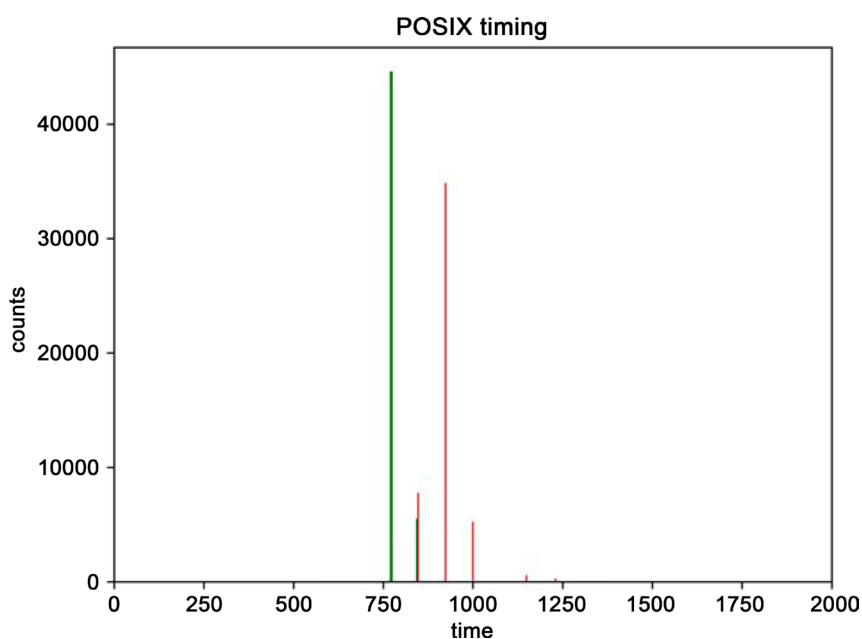
Figure 1. Cache hit and miss experiment
