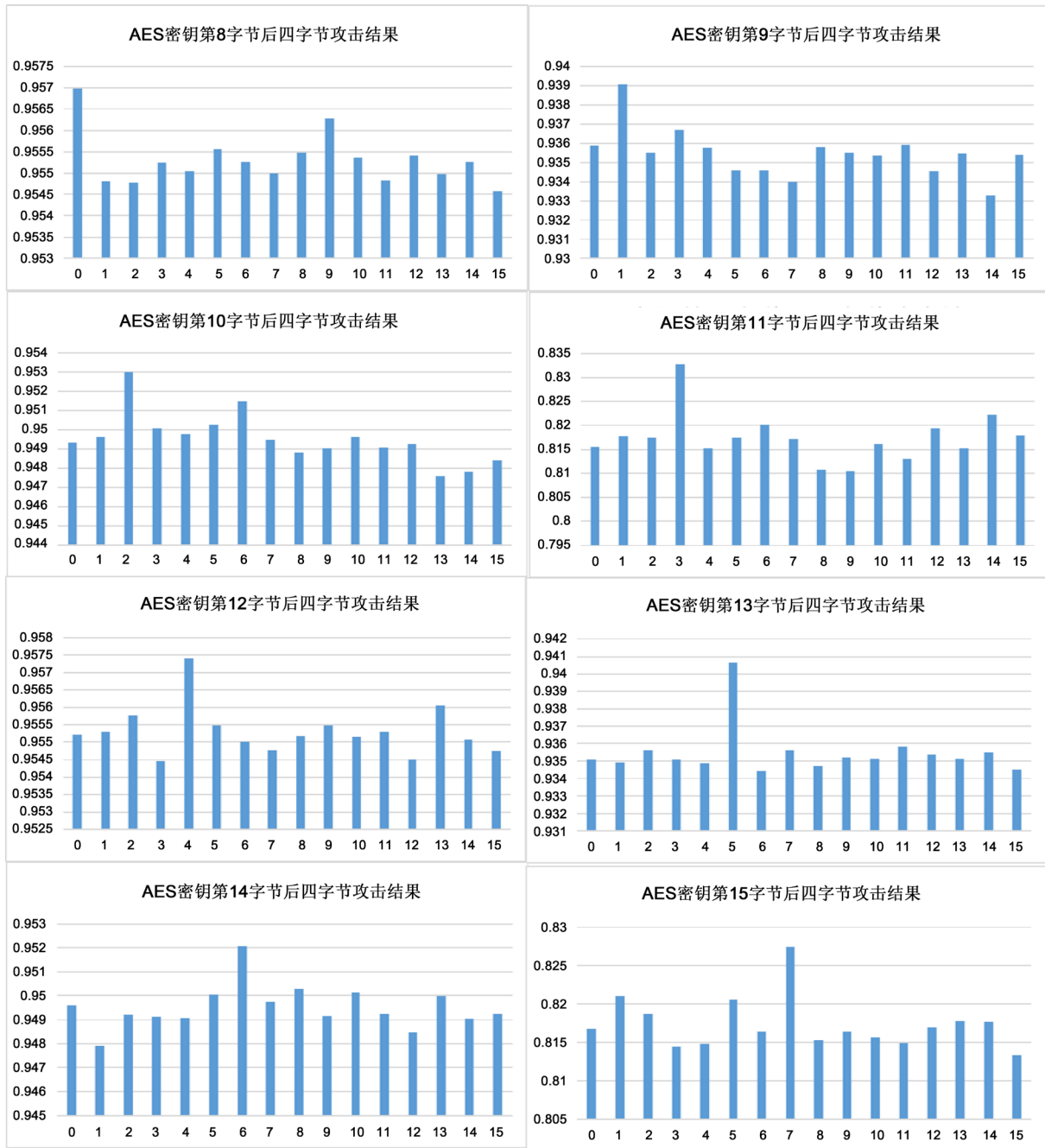
Figure 4. The result of AES last 8 bytes in first round attack 图 4. AES 第一轮攻击后 8 字节结果
