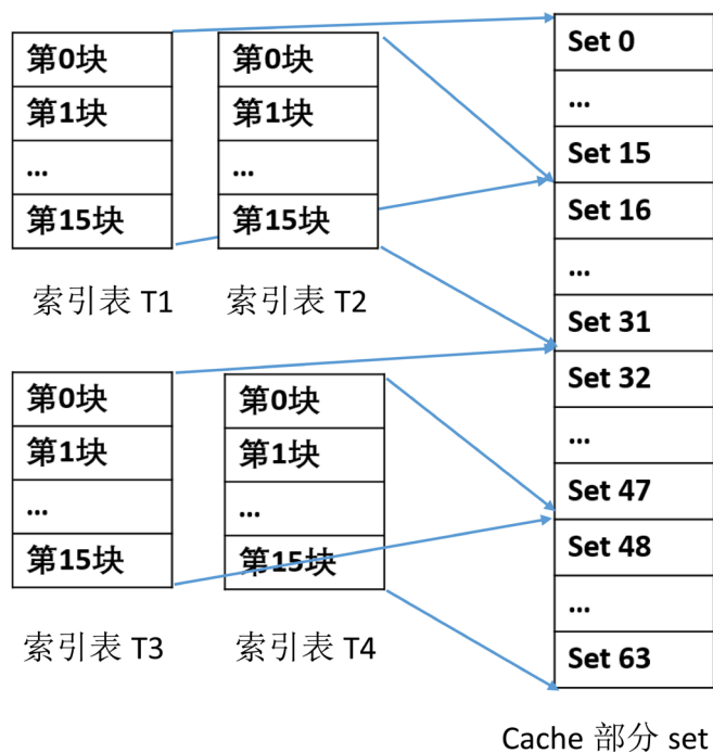
Figure 2. The map between AES table and Cache 图 2. AES 索引表与 Cache 映射情况
