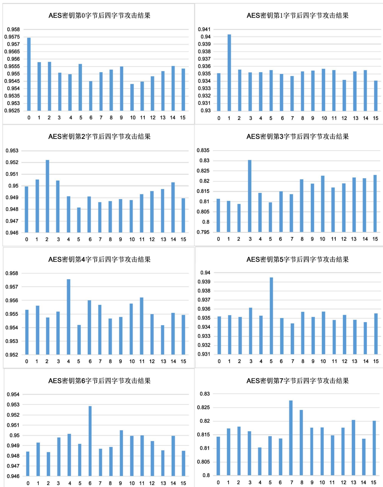
Figure 3. The result of AES first 8 bytes in first round attack
