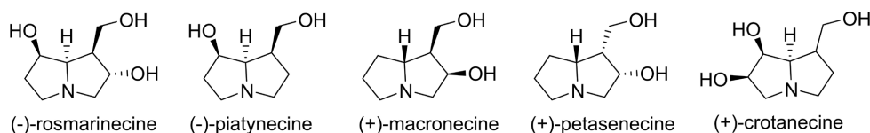
Figure 9. Pyrrolizidine biologicals
