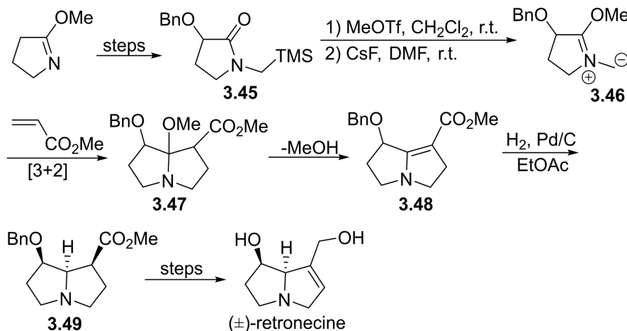
Figure 18. Synthesis of the pyrrolizidine alkaloid (±)-retronecine
