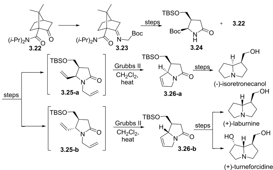
Figure 14. Synthesis of the pyrrolizidine alkaloids (-)-isoretronecanol, (+)-laburnine, and (+)-turneforcidine
