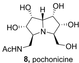
Figure 5. Pyrrolizidine alkaloid Pochonicine 图 5. 吡咯里西啉生物碱 Pochonicine
