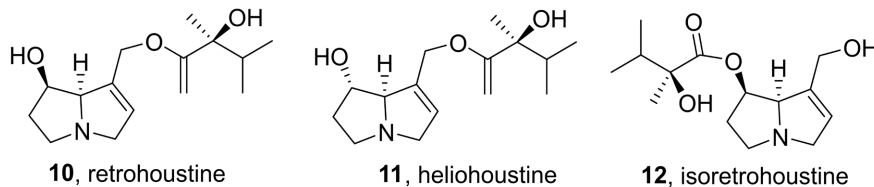
Figure 7. Pyrrolizidine alkaloid Retrohousine、Heliohousine and Isoretrohousine 图 7. 吡咯里西啉生物碱 Retrohousine、Heliohousine 和 Isoretrohousine
