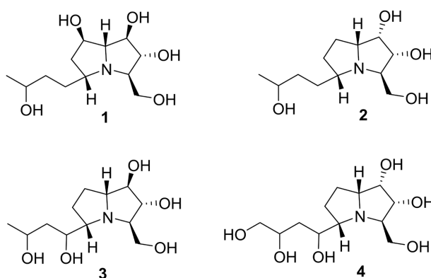
Figure 3. Pyrrolizidine alkaloid 图 3. 吡咯里西啶生物碱
