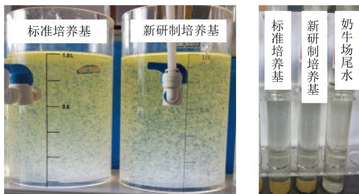
Figure 4. Floc formation and its settling effect 图 4. 絮体形成和沉降效果
