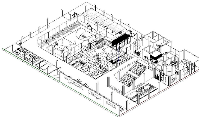
Figure 14. Landscape axonometric drawing 图 14. 景观轴测图
