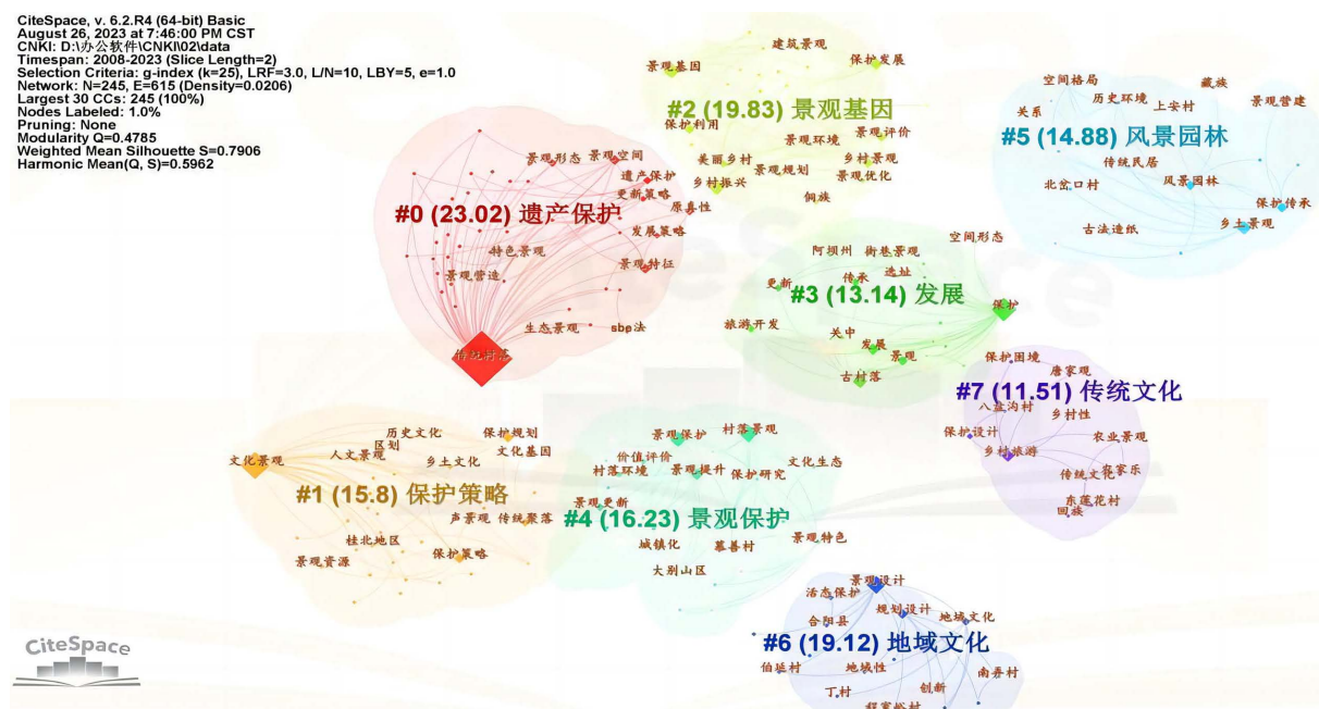
Figure 3. Keyword cluster atlas of traditional village protection research 图 3. 传统村落保护研究的关键词聚类图谱
