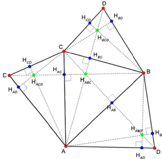
Figure 1. Symbolic expansion of point, line and surface projective coordinates 图 1. 点、线、面 3 态垂心坐标符号展开图
