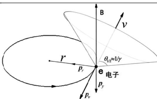
Figure 2. A schematic diagram of the decomposition of the momentum delivered by a radiated photon to the single electron 图 2. 辐射光子向单电子传递的动量分解示意图
