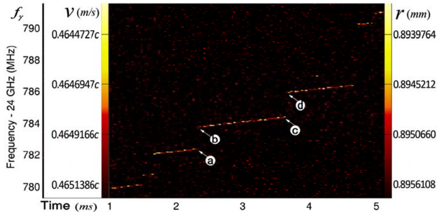
Figure 1. The change law of the single electron's position features in B = 1 (T) magnetic field with time 图 1. 单电子在 B = 1 (T) 的磁场中的位置特征随时间变化规律
