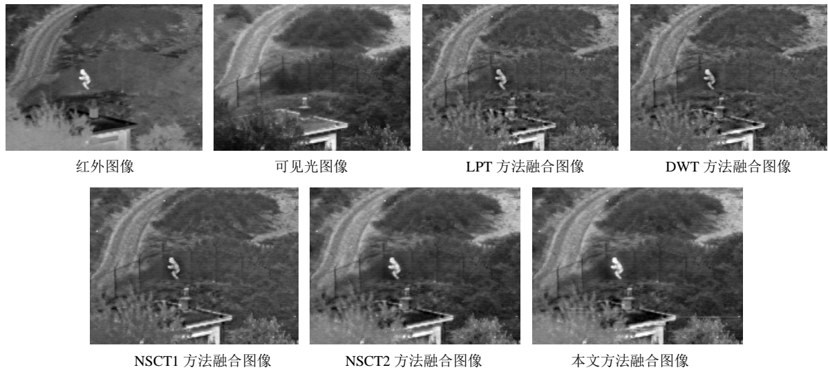
Figure 3. Simulation 2
