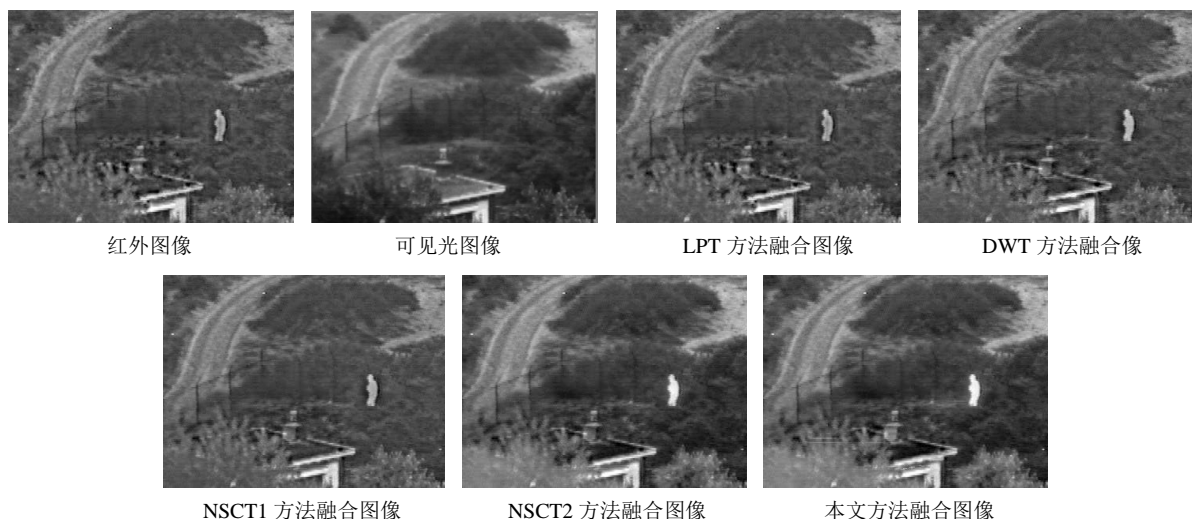
Figure 2. Simulation 1
