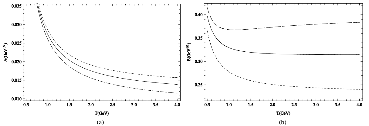
Figure 1. Variation of wave functions A and B with respect to the Borel parameter T at the momentum transfer q^2 = 0 \text{ GeV}^2 when choosing the chiral current. The dashed, solid and dotted curves correspond to the threshold s_0 = 1.4, 1.7, 2.0 \text{ GeV} respectively
