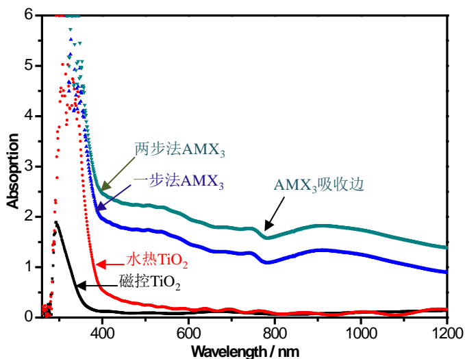
Figure 6. UV-vis absorption spectrum of different samples 图 6. 不同样品紫外可见光吸收光谱
