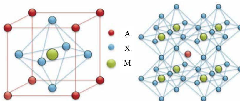
Figure 1. The crystal structure of perovskite materials [7]
