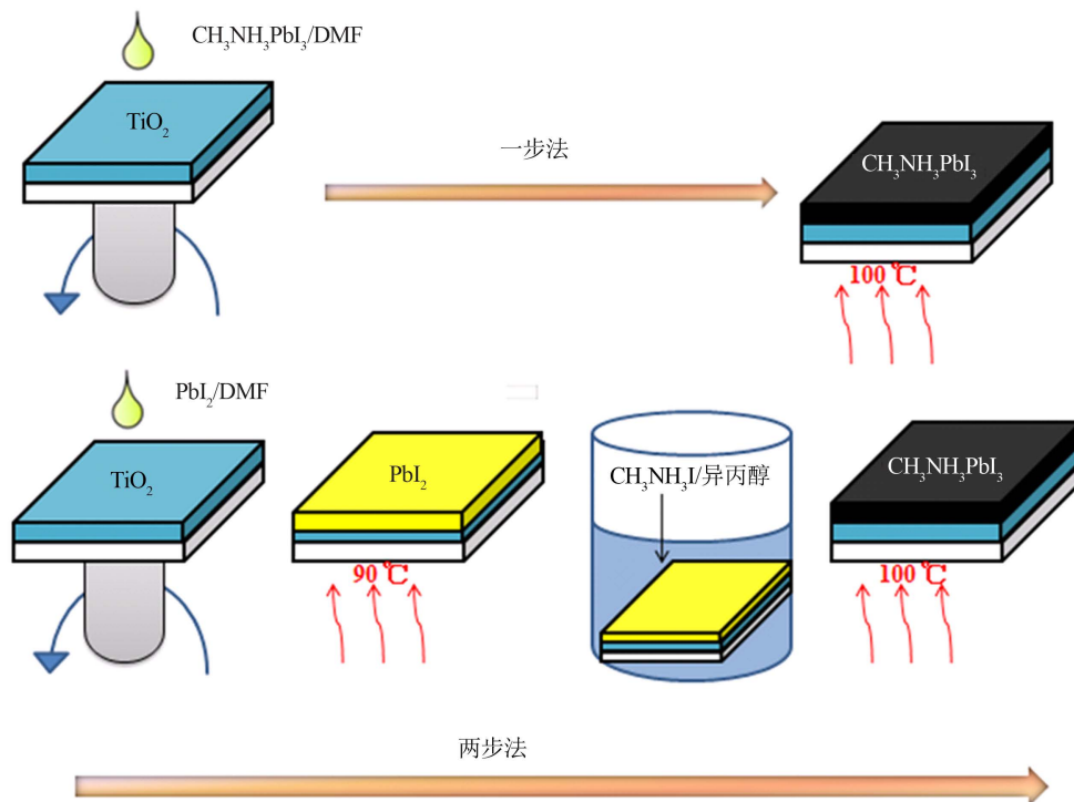
Figure 3. The schematic diagram of preparing \text{CH}_3\text{NH}_3\text{PbI}_3 via one-step and two-step method 图 3. 一步法，两步法制备 \text{CH}_3\text{NH}_3\text{PbI}_3 过程示意图
