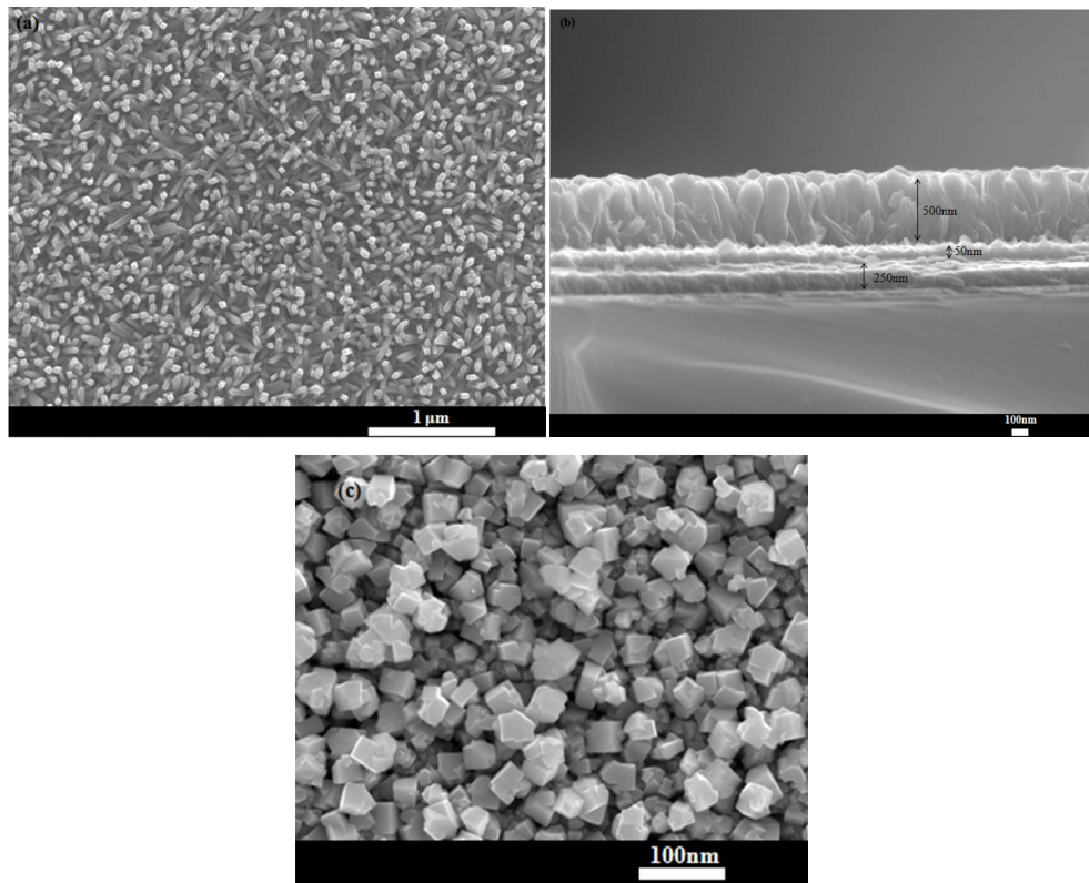
Figure 5. The SEM image of samples: (a) the surface topography of \text{TiO}_2 nanorod; (b) the cross-section image of \text{TiO}_2 nanorod; (c) the surface topography of \text{CH}_3\text{NH}_3\text{PbI}_3 图 5. 样品扫描电镜图: (a) \text{TiO}_2 纳米棒表面形貌图; (b) \text{TiO}_2 纳米棒截面图; (c) \text{CH}_3\text{NH}_3\text{PbI}_3 表面形貌图
