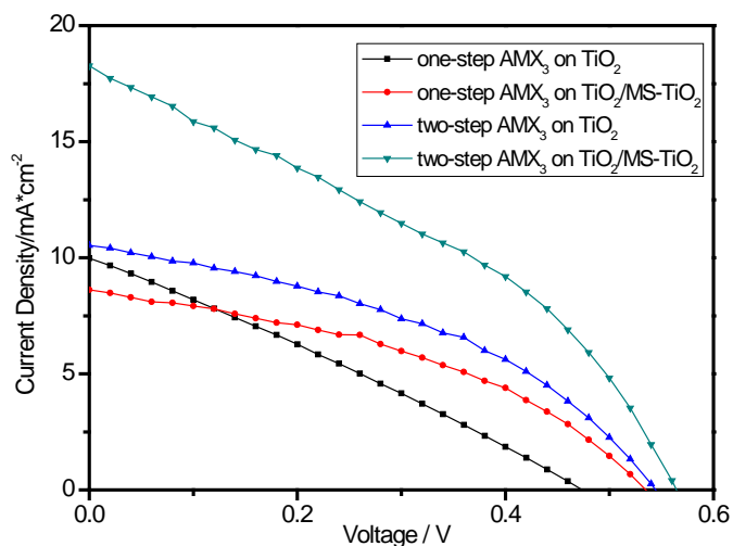
Figure 7. The current density-voltage image of solar cells assembled by different electron transport layers and perovskite layers 图 7. 不同电子传输层及钙钛矿层组装电池的光电流密度-电压图
