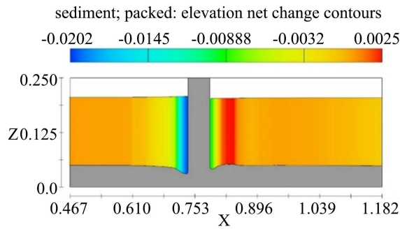
Figure 3. Longitudinal section of bridge abutment at t = 300 s 图 3. t = 300 s 时桥墩纵向剖面
