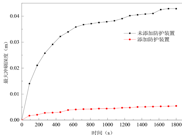
Figure 15. Time history curve of maximum scour depth before and after protection 图 15. 防护前后最大冲刷深度时程曲线
