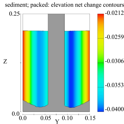
Figure 10. Transverse section of bridge abutment at t = 1800 s 图 10. t = 1800 s 时桥墩横向剖面
