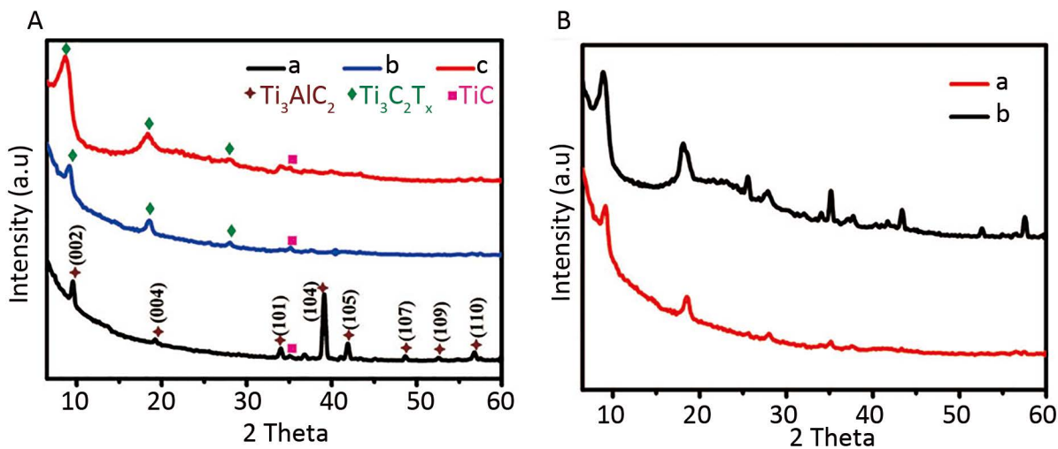
Figure 4. XRD patterns for Ti_3AlC_2 and Ti_3C_2T_x , in figure of (A) a for Ti_3AlC_2 , b for Ti_3C_2T_x obtained by reacting with 40% HF, c for Ti_3C_2T_x obtained by reacting with 50% HF; in figure of (B) a for Ti_3C_2T_x obtained by reacting with 40% HF for 60 h, b for 80 h
