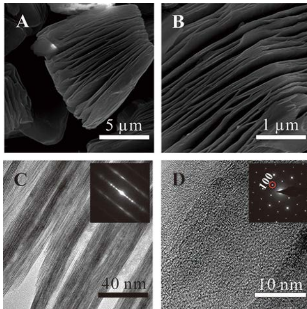
Figure 3. (A)-(B) SEM images for Ti_3AlC_2 reacting with 50% HF for 24 h under 50^\circ C , (A) low-magnification SEM image, (B) high-magnification SEM image; (C)-(D) TEM images for Ti_3AlC_2 reacting with 50% HF for 24 h under 50^\circ C , (C) low-magnification TEM image, (D) high-magnification TEM image, the corresponding electron diffraction patterns are shown in inset of the figures
