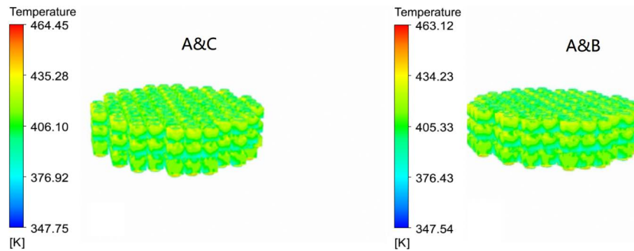
Figure 6. Temperature contour on the surface of the coil assembly
